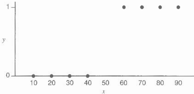
FIGURE 5.6 Perfect discrimination resulting in infinite logistic regression parameter estimate.
